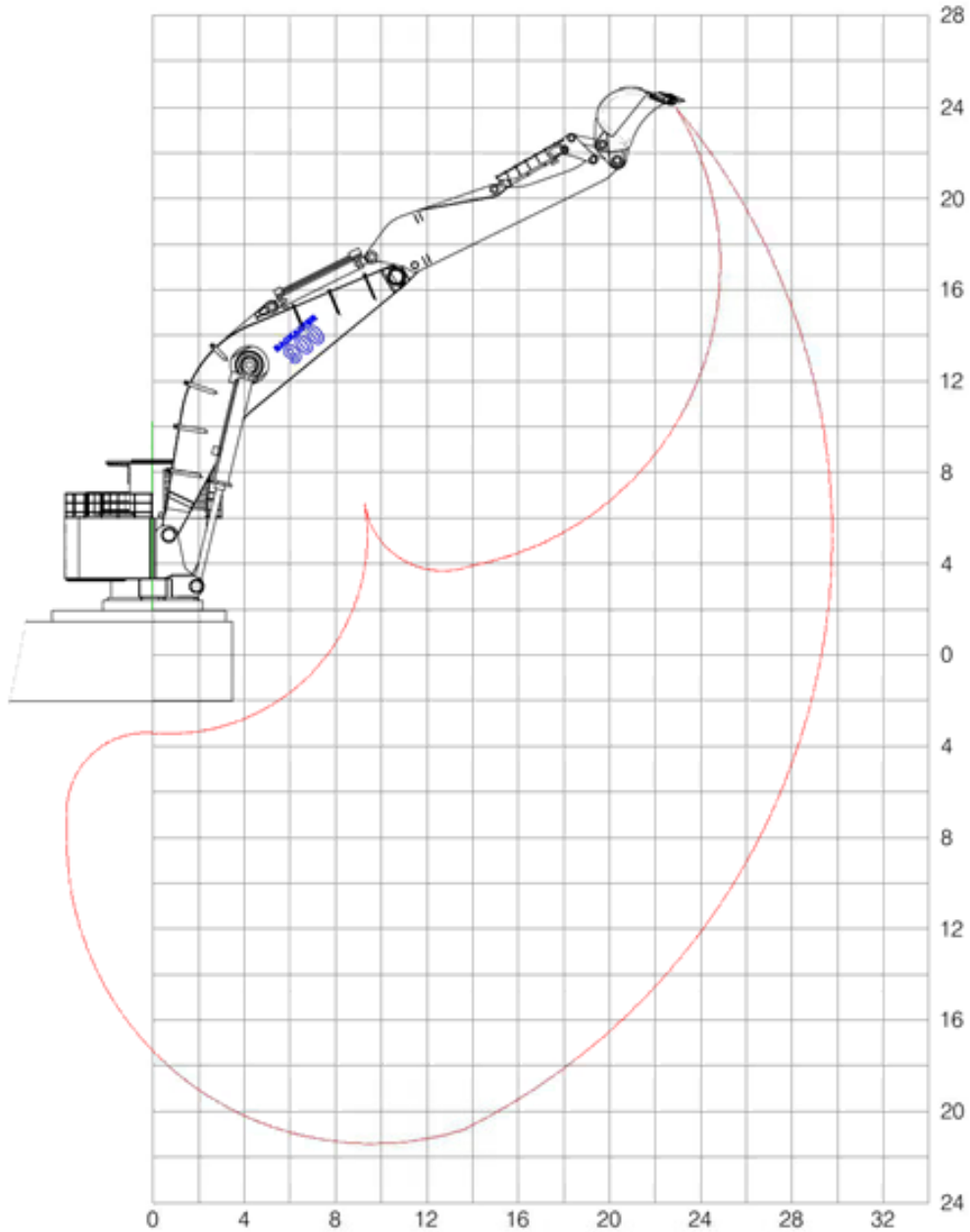
Dredging Diagram
